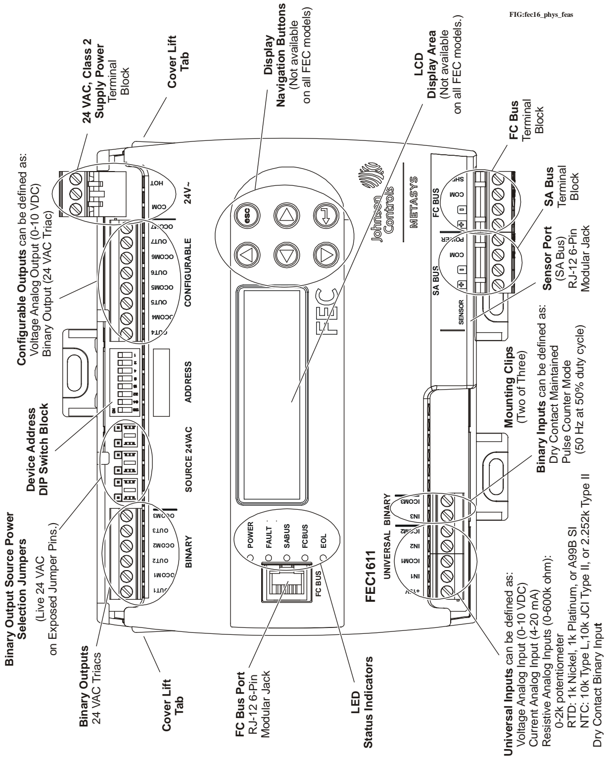
Figure 3: FEC1611 Controller Physical Features and Wiring Terminals
